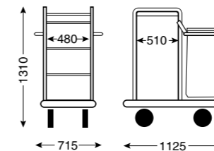
CHARIOT IBIZA 9 995 10 54
